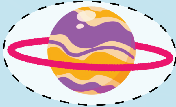
Saturn
