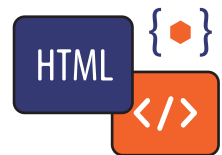
Programming Language
