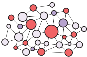
Algorithm
